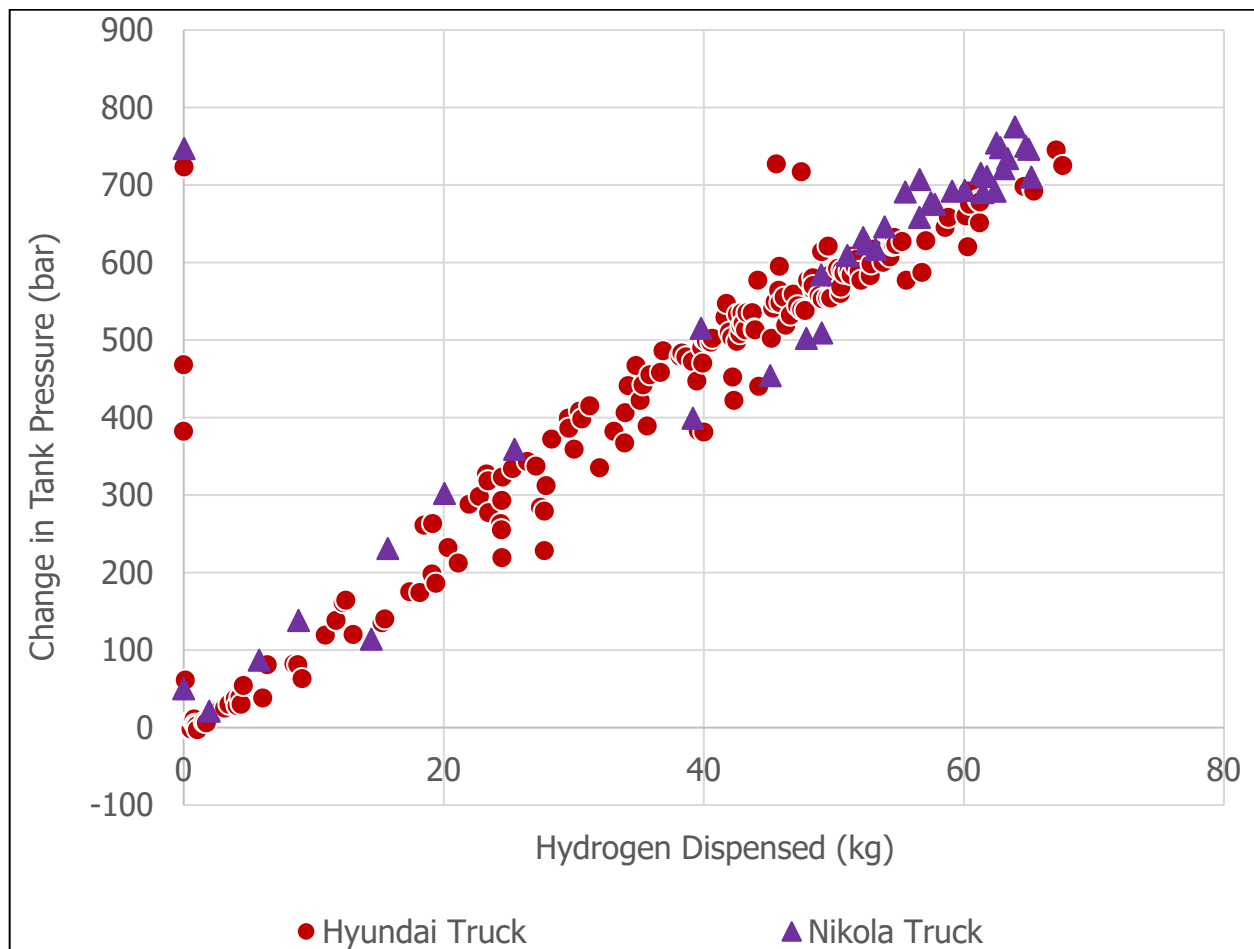
Figure 6: Change in Pressure vs. Hydrogen Added for Conjoined Fills
