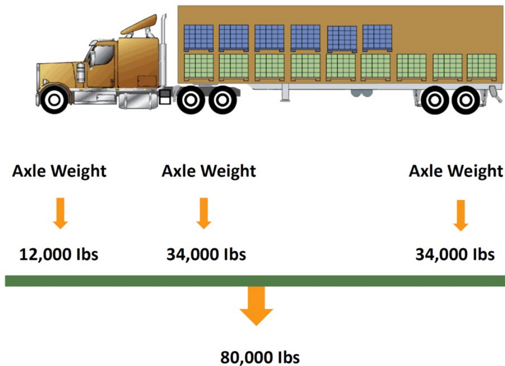
Figure 4: Overview of American axel loading limits 40
