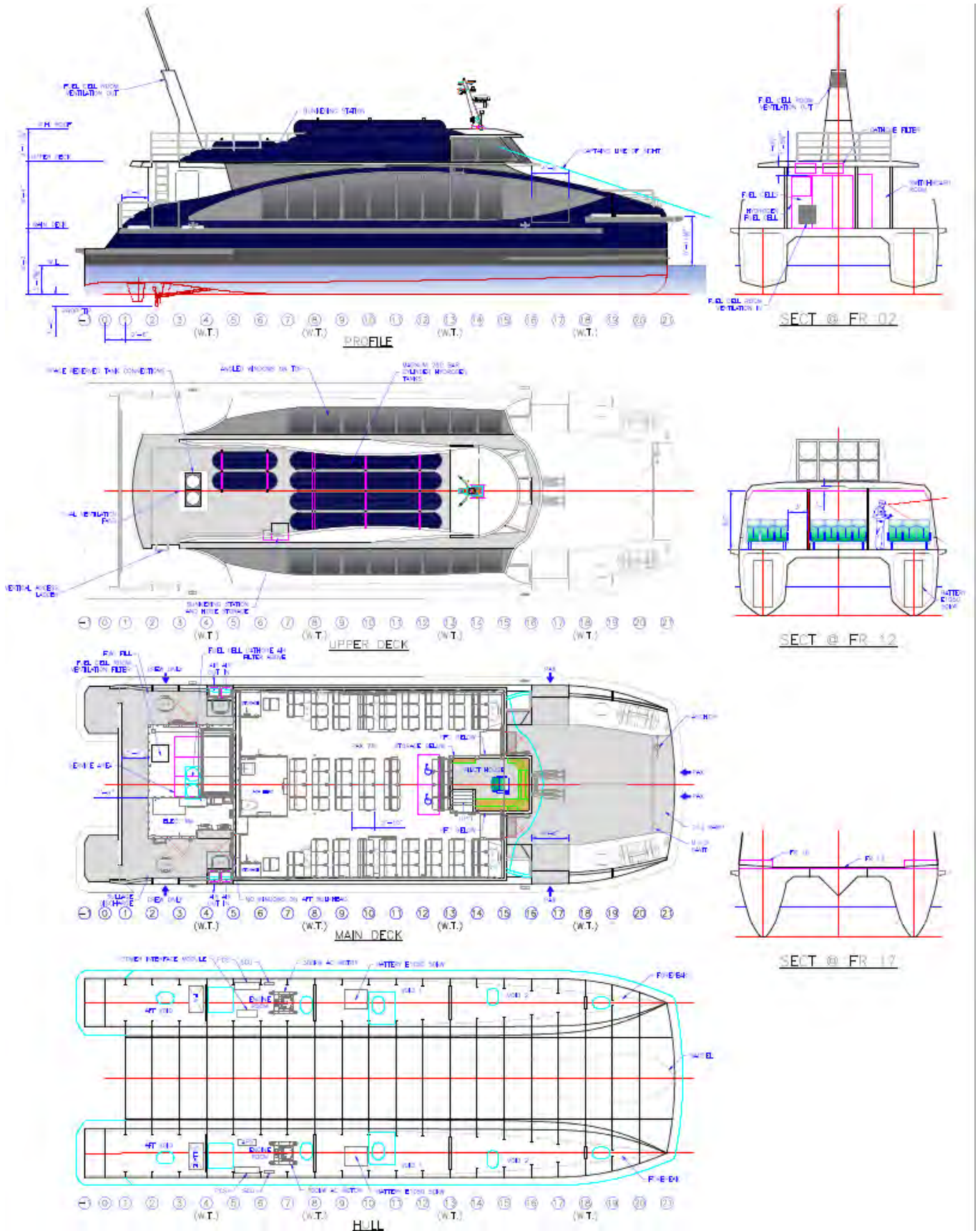
Figure #4 - Sea General Arrangement
