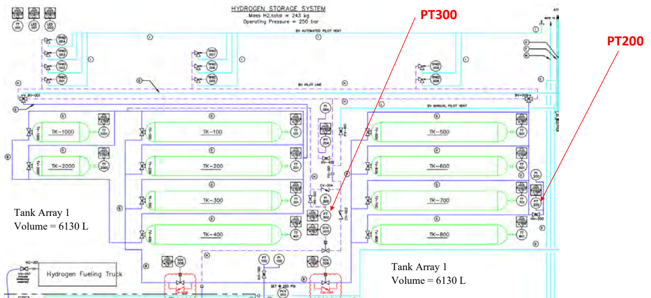
Figure #1 - Sea Change Hydrogen Tank Diagram
