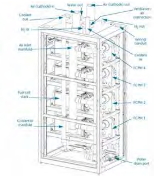
Hydrogen Fuel Cell Rack Diagram
